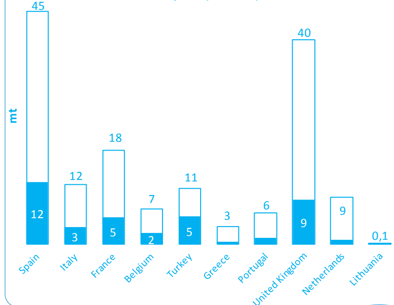
Regasification capacity use in Europe (2014)
